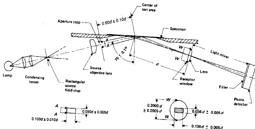
Fig. 1. Schematic drawing of glossmeter in which dimensions are given in terms of d , the distance between center of test area and receptor window. The cross-hatched rectangle in the W-W circle represents the image of the source field stop in the receptor window.
